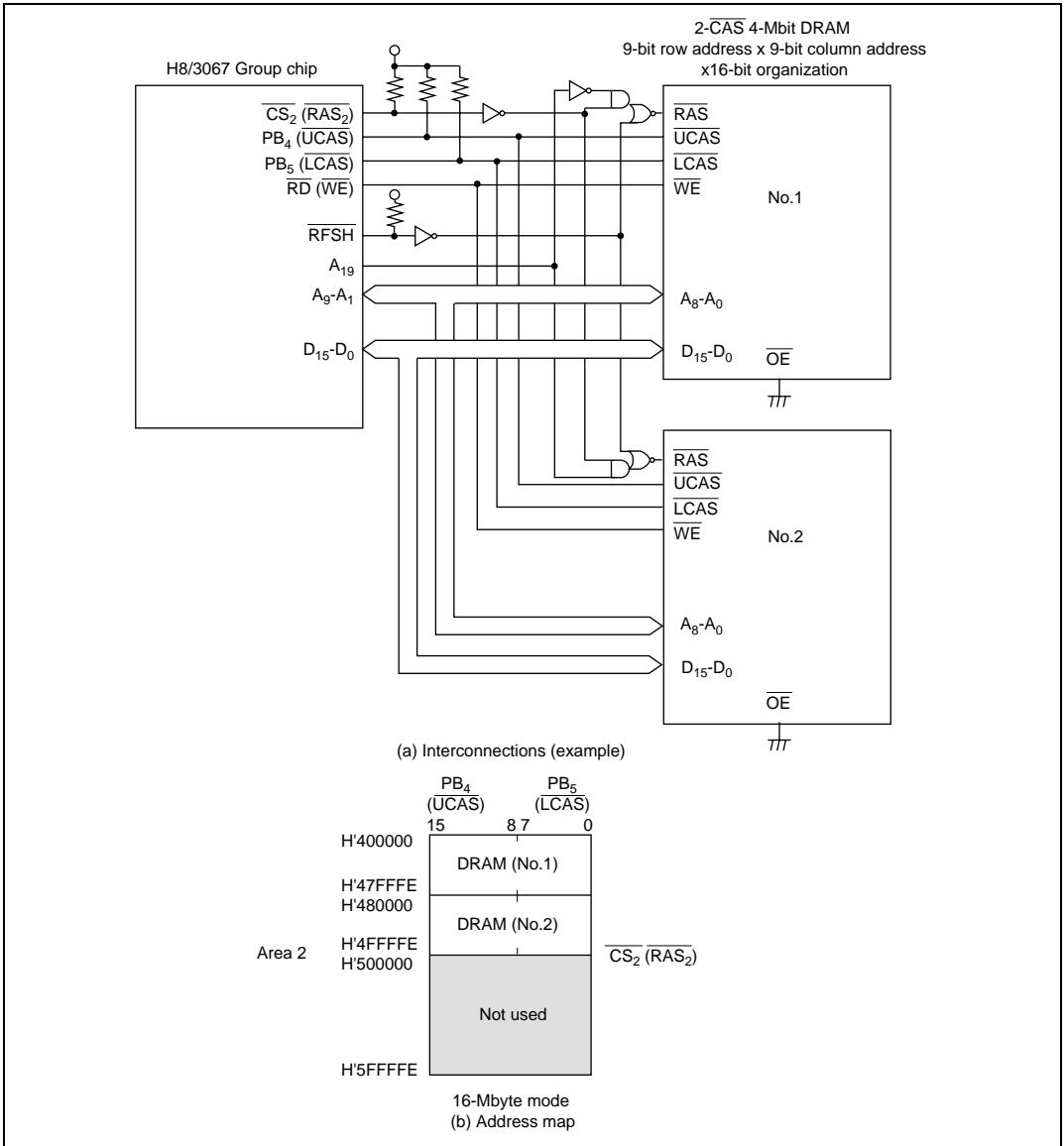
Figure 6.33 Interconnections and Address Map for 2-CAS 4-Mbit DRAMs with x16-Bit Organization
