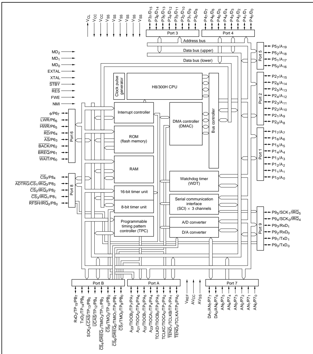
Figure 1.1 Block Diagram
